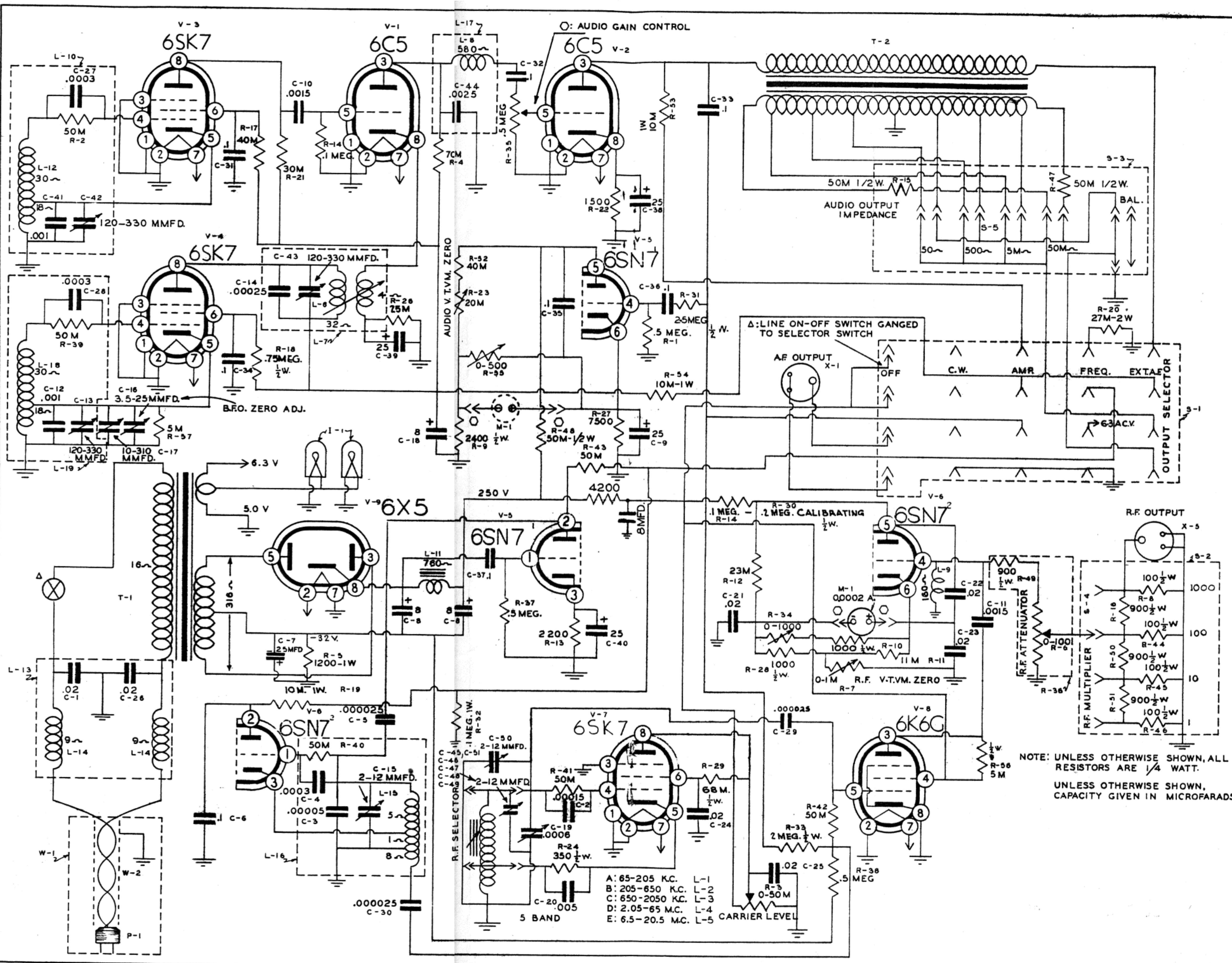
SCHMATIC WIRING DIAGRAM SUPREME MODEL 666 A.F. AND R.F. OSCILLATOR
