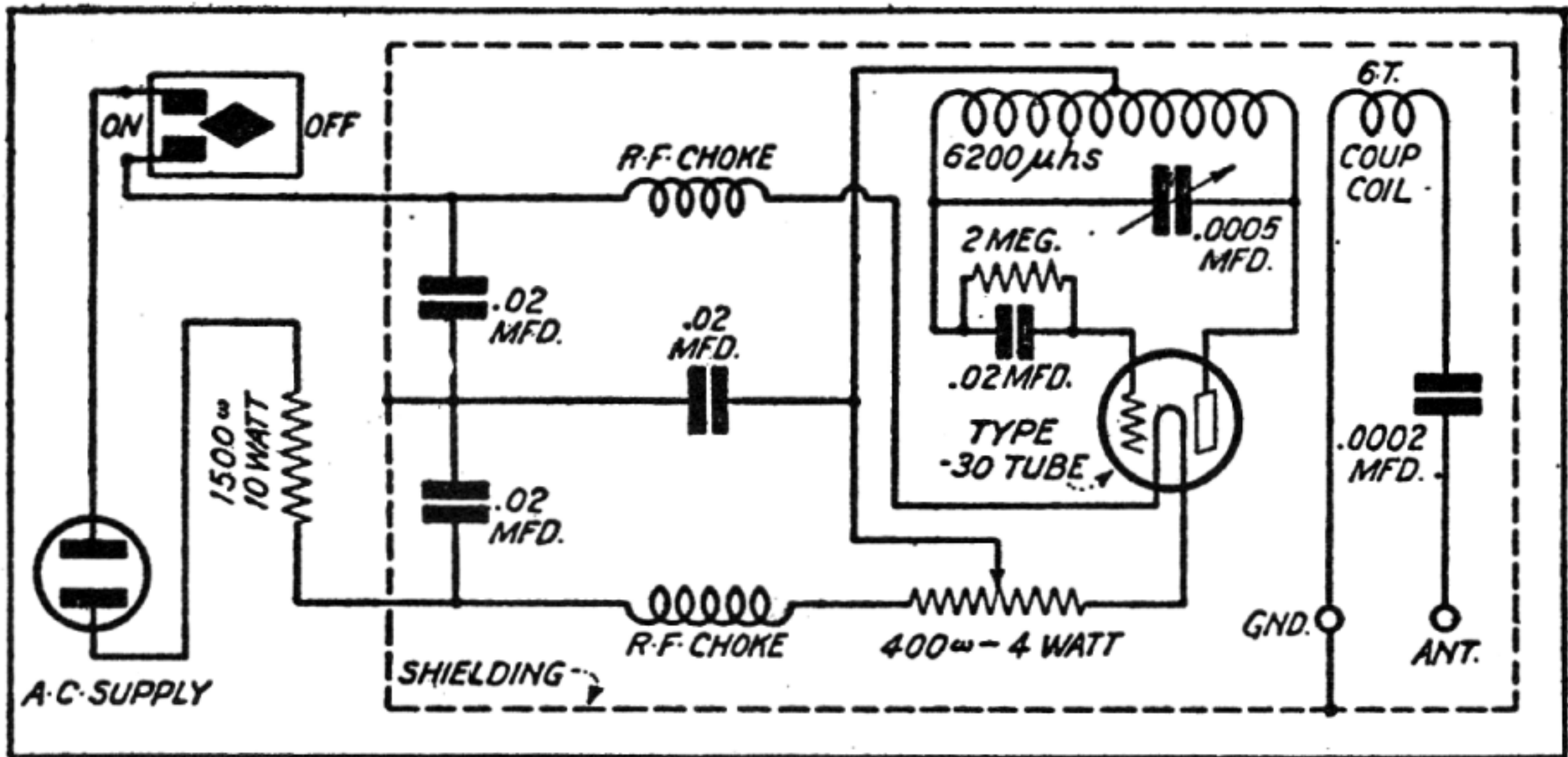
Model 60 Oscillator
